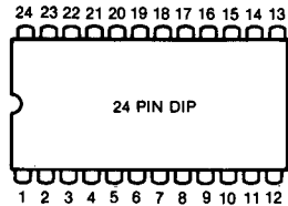
Fig. D-6. 24-pin dual in-line package.
